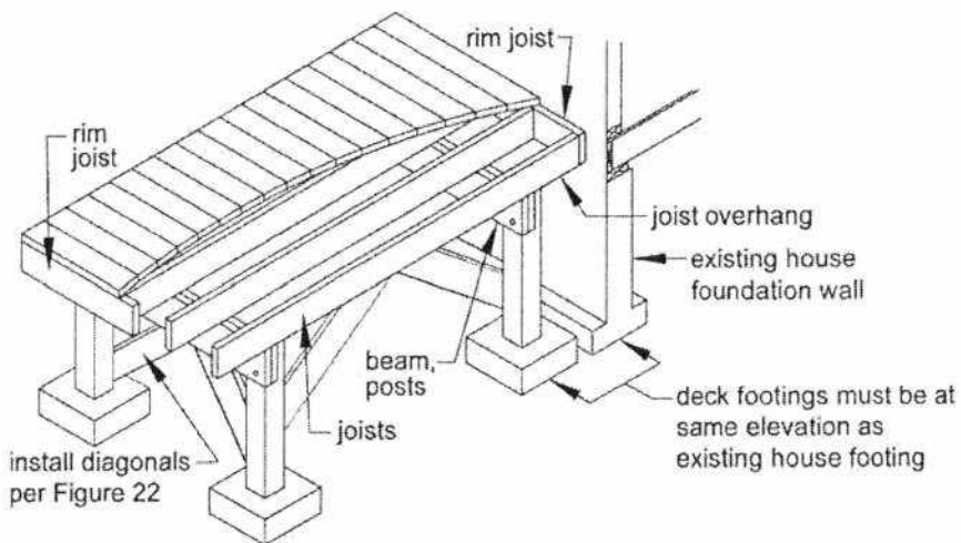
Figure 21: Free-Standing Deck
