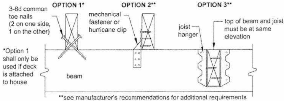
Figure 6: Joist-to-Beam Detail
